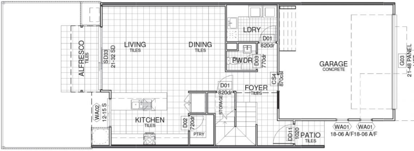
1 LOWER FLOOR
