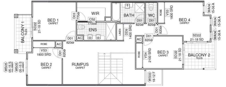
2 UPPER FLOOR
