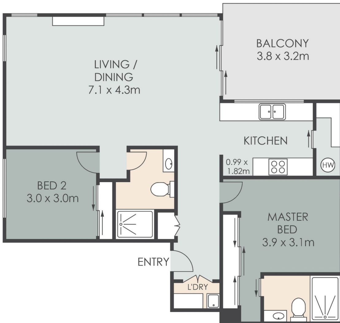
UPPER LEVEL
